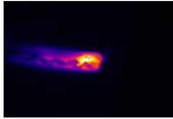
PA6 GF30 - PA6 GF30: Kare uç, 20 mm/dak, 1250 dev/dak, 176.62°C
