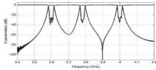
Figure 3. Structure of triple band rectangular waveguide (a) and measurement results(b)(Zhu et al., 2016).
