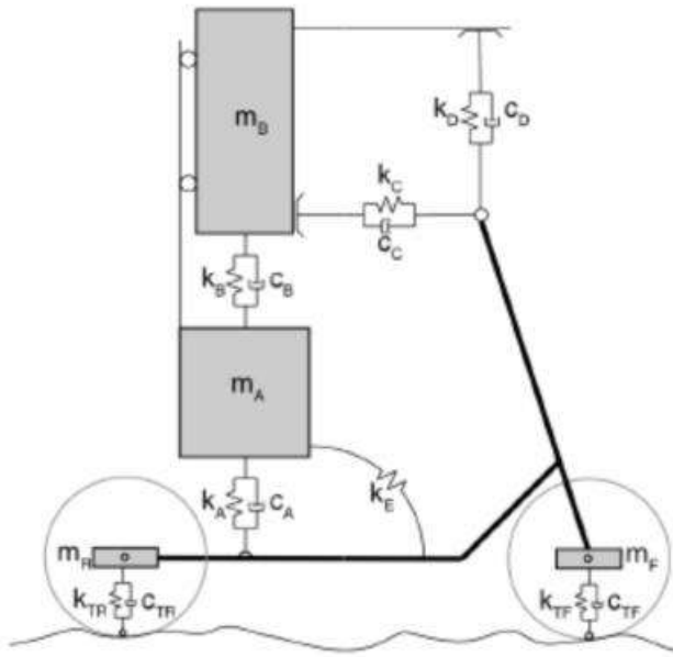
Fig 1. Physical model of e-scooter and driver (Asperti et al., 2021).
