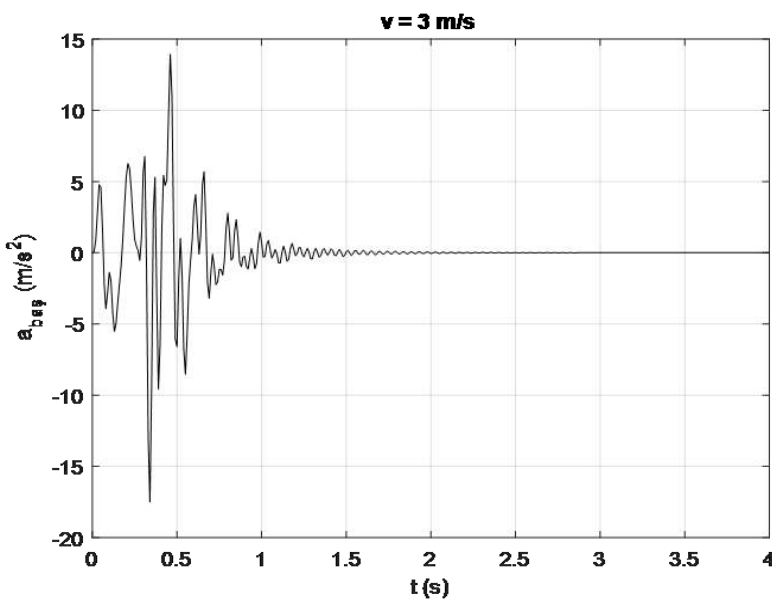
Fig 3. When the scooter speed is taken as 3 m/sec, the vertical accelerations occurring.
