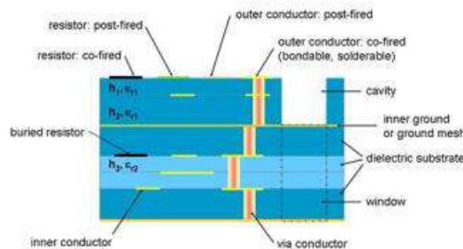
Figure 8. General structure of LTCC technology (Wolff, 2007).
