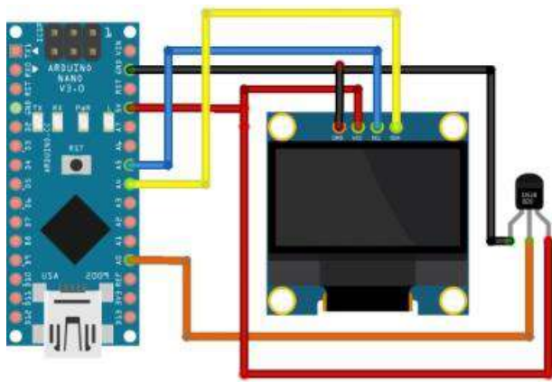
Figure 5. Electronic circuit designed for body temperature measurement.
