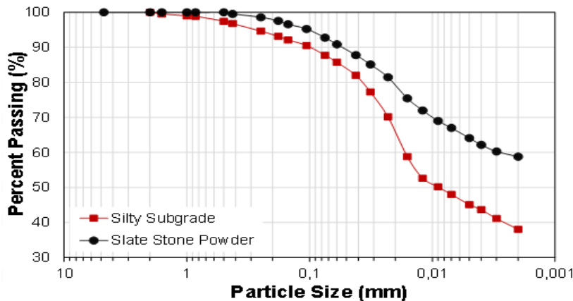
Figure 1. Particle size distribution of soil and SSP
