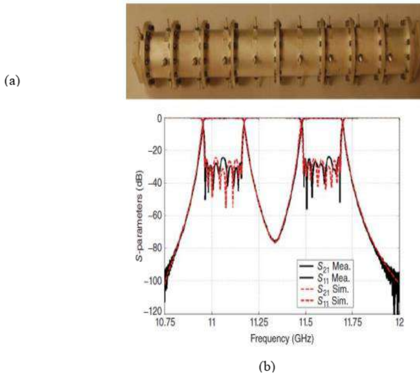
Figure 2. Structure of dual-band waveguide filter (a) and measurement results (b) (L. Zhu et al., 2017).
