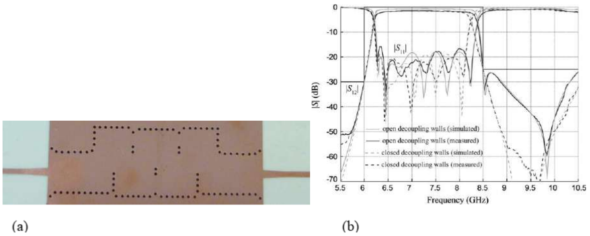
Figure 5. Structure of single band SIW (a) and measurement result (b) (Mira et al., 2009).
