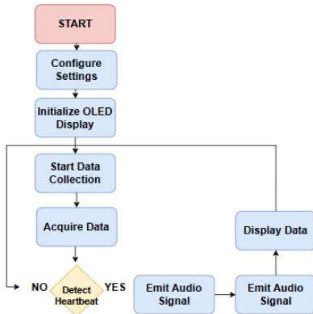
Figure 9. Software flowchart developed for SpO 2 and BPM.
