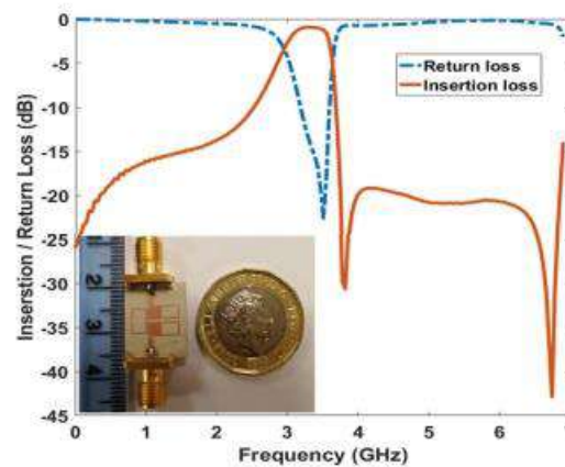
Figure 11. Planar microstrip structure and measurement result (Al-Yasir et al., 2019)
