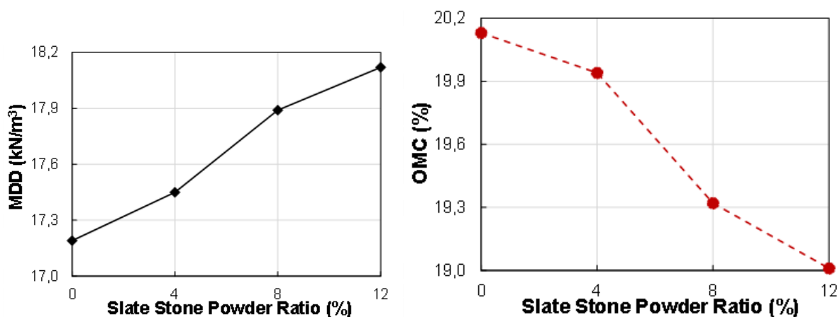
Figure 2. Change in the MDD and OMC values of soil with different SSP ratios
