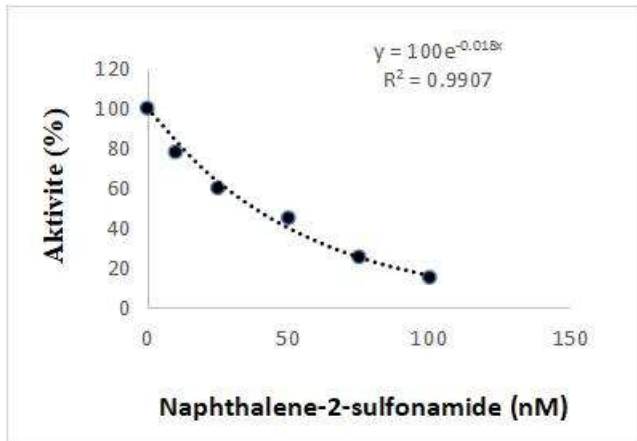
Figure 1. The % Activity-Concentration Graph Obtained with Naphthalene-2-sulfonamide for the MPO Enzyme Using O-Dianisidine Substrate
