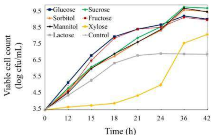
Figure 1. Growth curves of M. pulcherrima .
