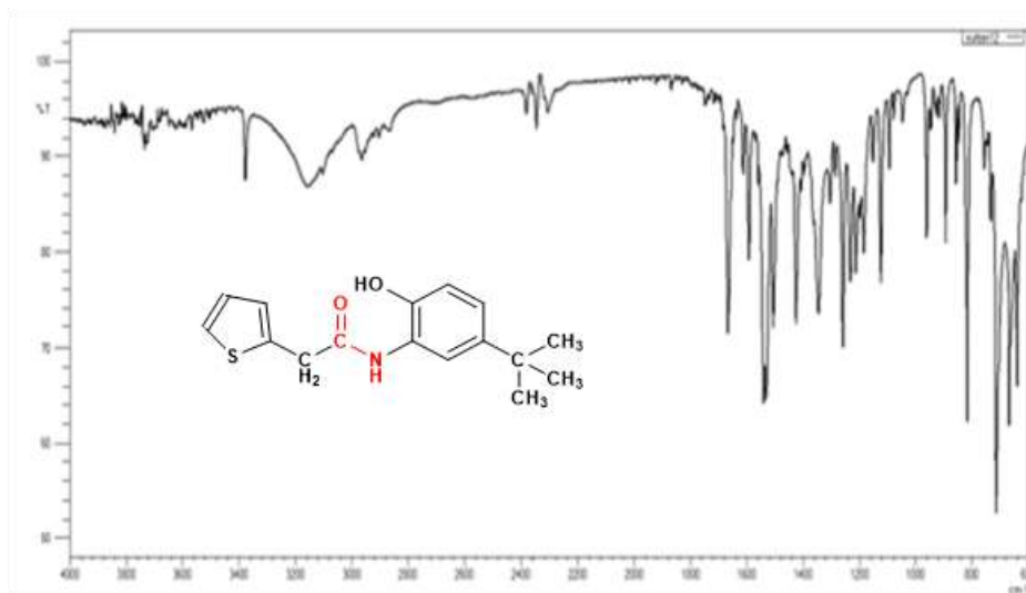
Figure 2. FT-IR spectrum of the TBHPT-Ac.
