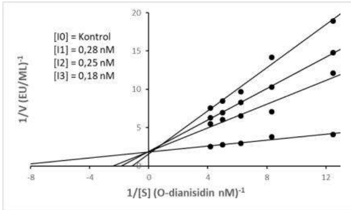
Figure 4. O-Dianisidine as the Substrate with 4-Nitrobenzenesulfonyl chloride to Obtain the 1/V-1/[S] Graph for MPO Enzyme
