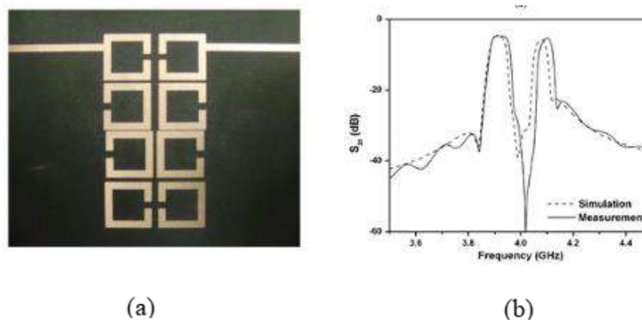
Figure 12. Stripline structure for the dual-pass band filter (a) and measurement result (b) (Lee & Sarabandi, 2007)
