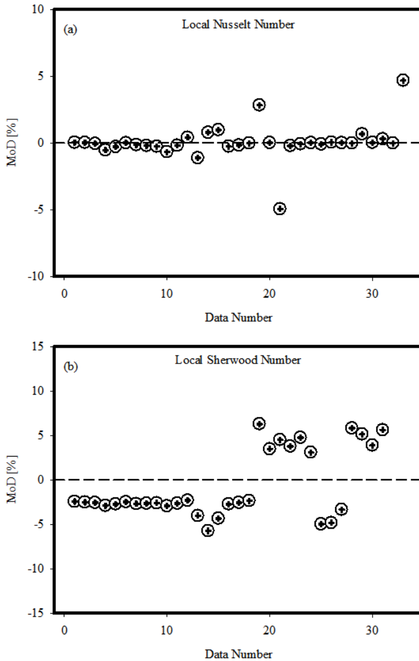
Figure 2. MoD values for both ANN models
