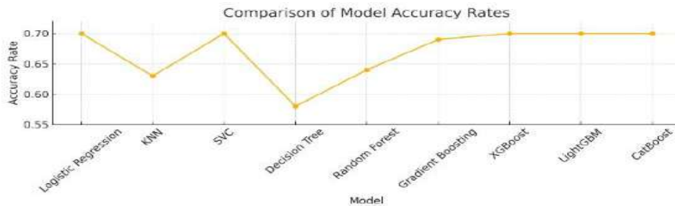
Figure 12. Comparison of model accuracy rates.
