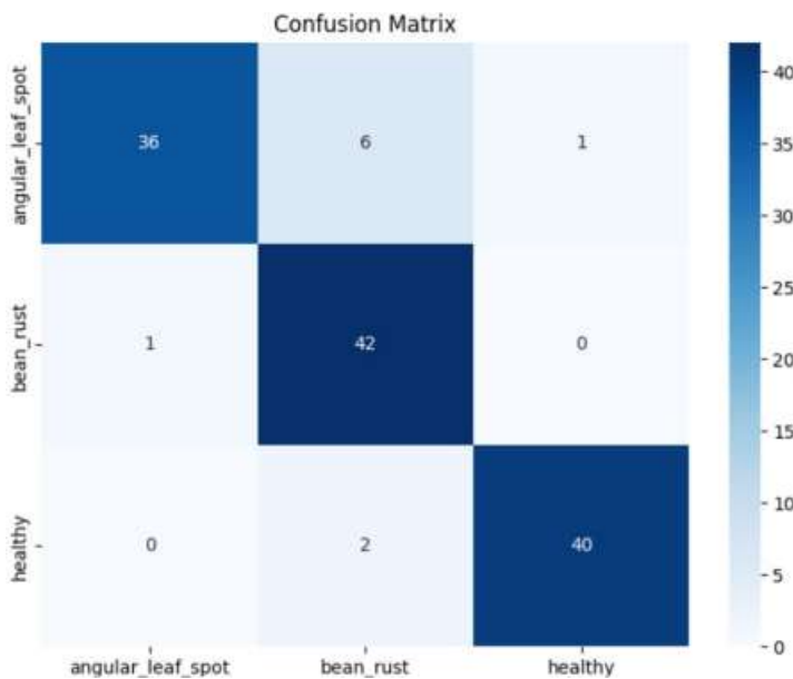
Figure 3. Confusion matrix of the test results for the lightweight CNN model.
