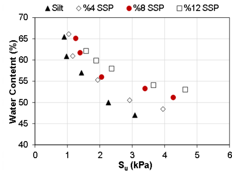
Figure 3. Change in the S_u of soil with different SSP and water content
