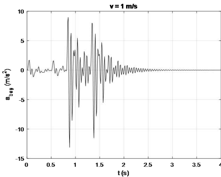
Fig 2. When the scooter speed is taken as 1 m/s, the vertical accelerations occurring.
