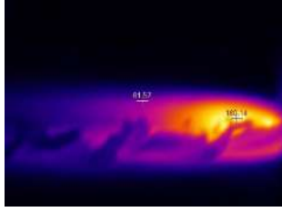
ABS Plus- ABS Plus: Üçgen Uç 20 mm/dak, 1250 dev/dak, 180.14°C
