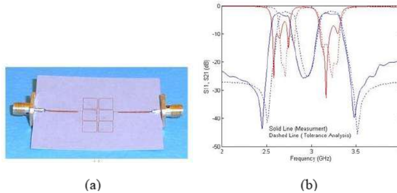
Figure 13. Planar structure for dual band filter (a) and measurement result (b) (Mokhtaari et al., 2006).
