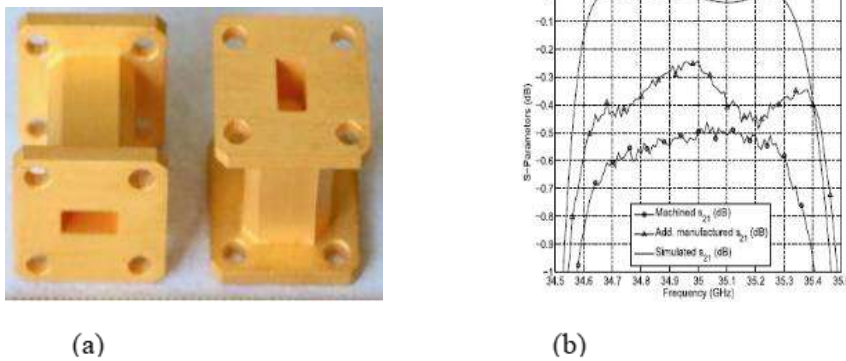
Figure 1. Structure of rectangular waveguide filter (a) and measurement results (b) (Kelleci & Atalar, 2017).
