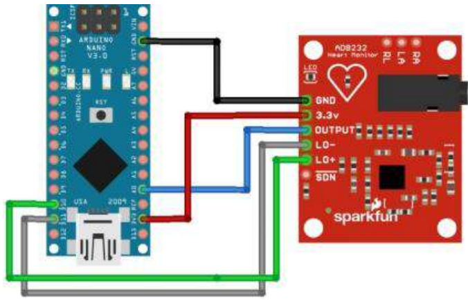
Figure 3. ECG control board assembly.
