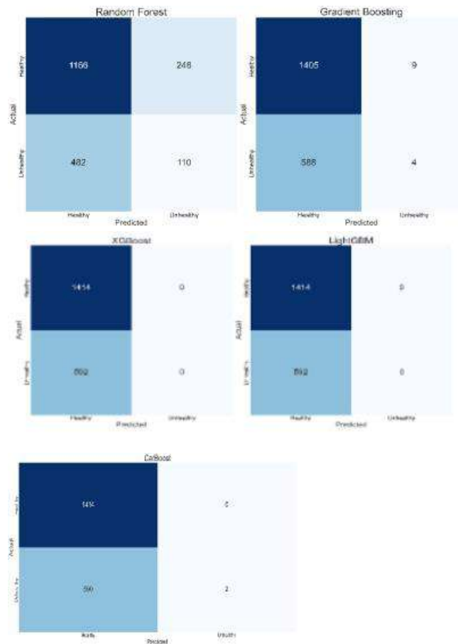
Figure 11. Confusion matrix representations of models.
