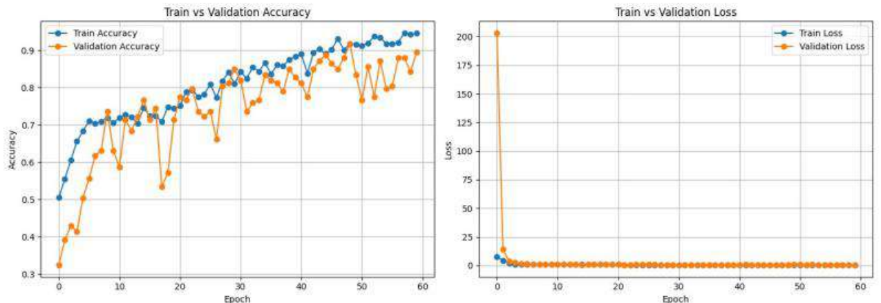
Figure 2. Training and validation accuracy and loss curves of the lightweight CNN model
