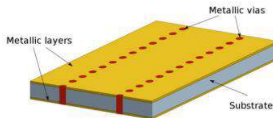
Figure 4. General structure of SIW (Nwajana & Obi, 2022).
