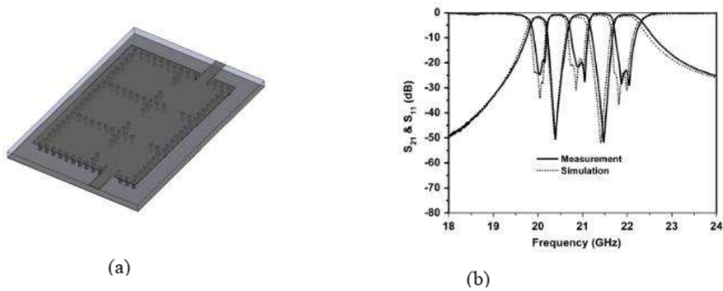
Figure 7 Structure of triple-band SIW (a) and measurement result (b) (X. Chen et al., 2007).
