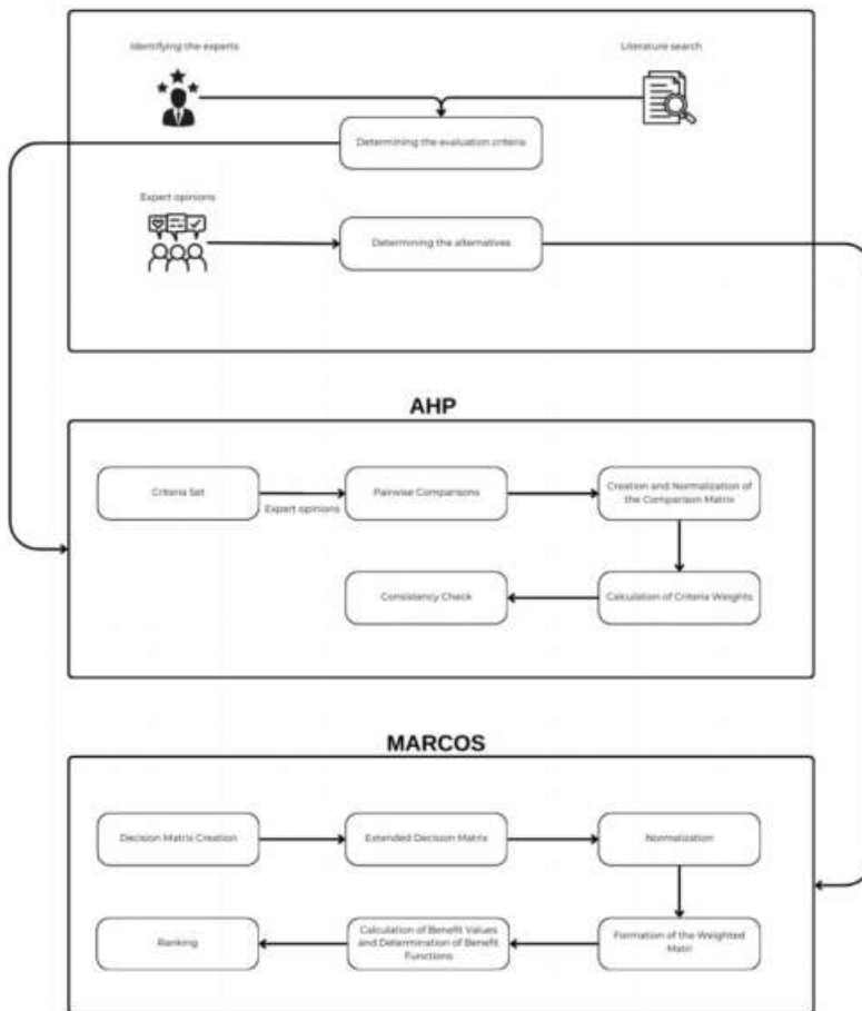
Figure 1. Method Flowchart
