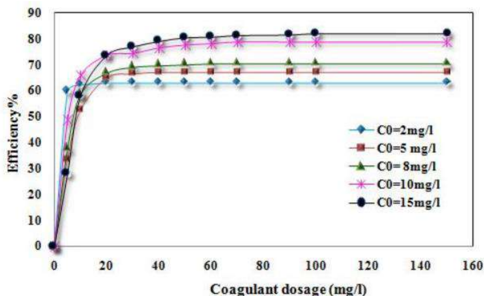
Figure 2: Aluminum sulphate dosage effect on various acetaminophen concentrations C_0 removal in distilled water at pH 7.
