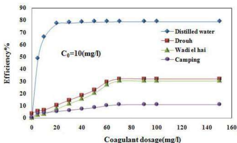
Figure 3 : Evolution of removal yields of acetaminophen depending on the coagulant dosage in various mineralied waters( C_0= 10\text{mg/l} )
