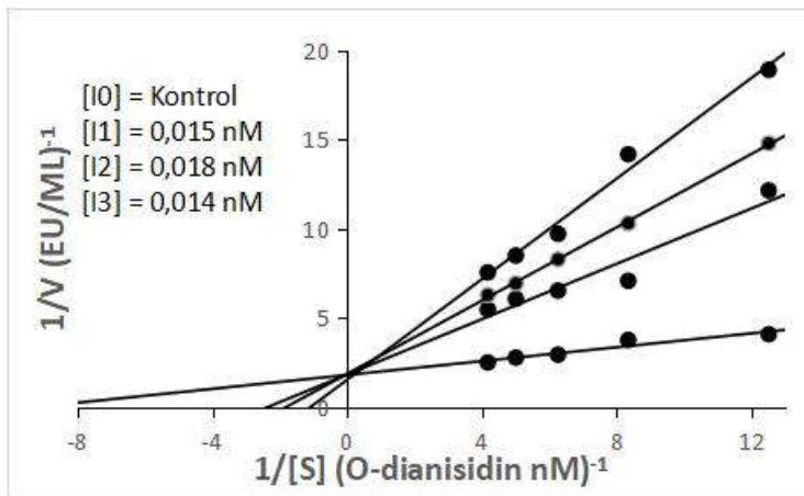
Figure 2. The 1/V-1/[S] Graph Obtained with Naphthalene-2-sulfonamide in the Presence of O-Dianisidine Substrate for the MPO Enzyme
