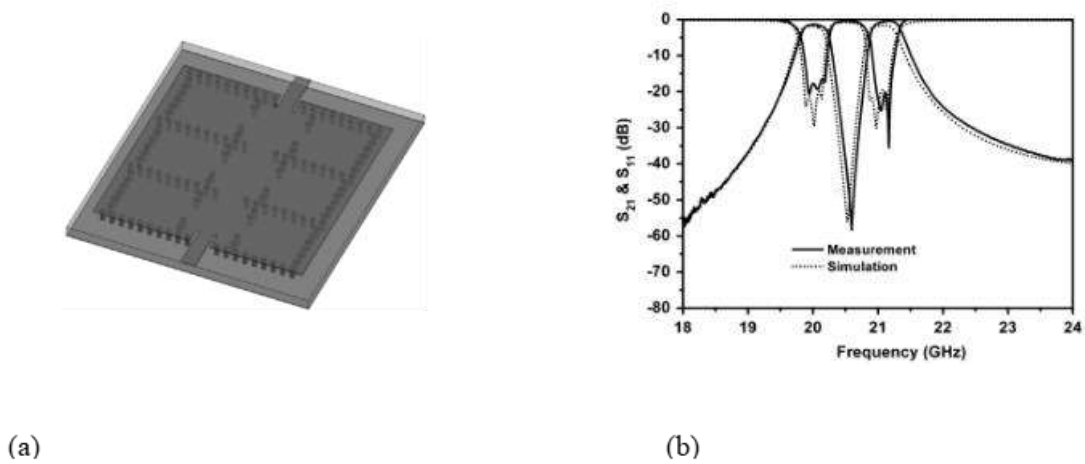
Figure 6 Structure of dual-band SIW (a) and measurement result (b) (X. Chen et al., 2007).
