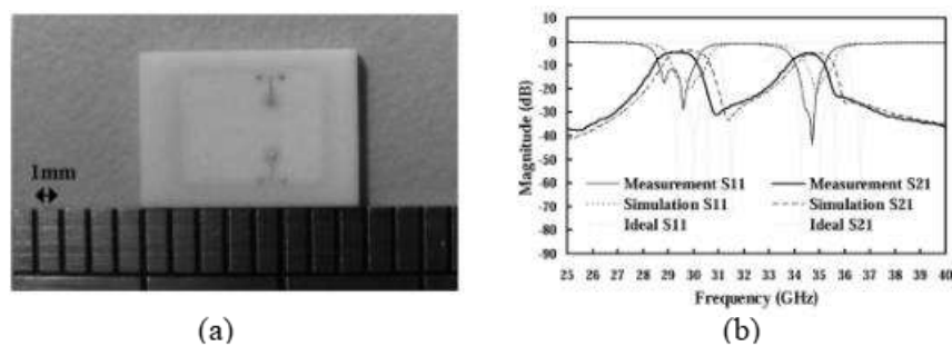
Figure 10. Structure of dual band LTCC filter and measurement result (Chen et al., 2009).
