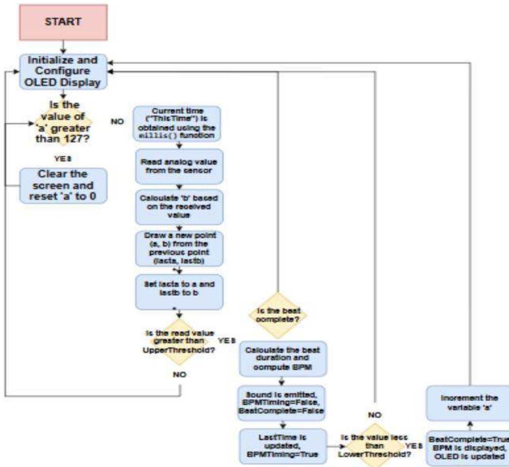
Figure 7. Software flowchart to be developed for EKG data.
