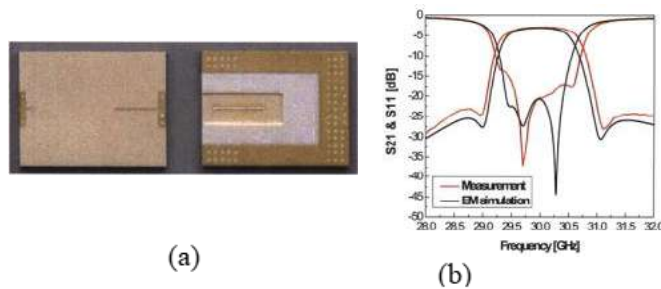
Figure 9. Structure of single band LTCC filter (a) and measurement result (b) (Ahn & Yom, 2008).
