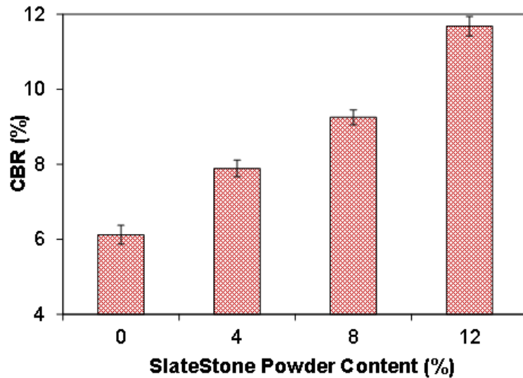
Figure 4. Change in the CBR value of soil with different SSP content
