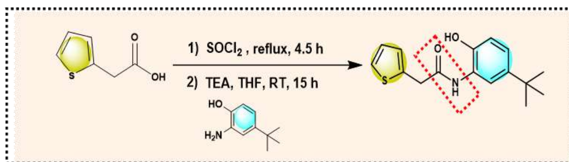
Figure 1. Synthetic route for the new TBHPT-Ac.
