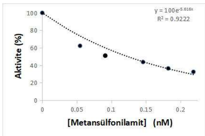
Figure 7. The Percentage Activity-Concentration Graph Obtained with Methanesulfonamide as Dependent on O-Dianisidine Substrate for MPO Enzyme
